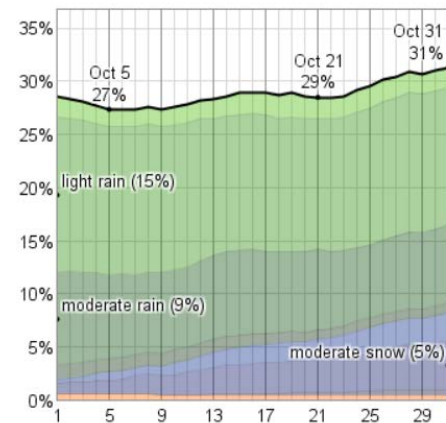
Probability of Precipitation at Some Point in the Day in October
