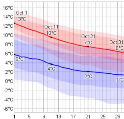
Daily High and Low Temperature in October
