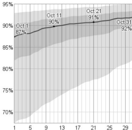
Median Cloud Cover in October
