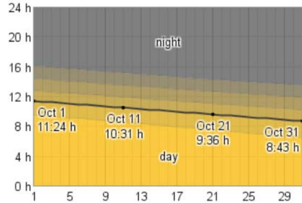
Daily Hours of Daylight and Twilight in October
