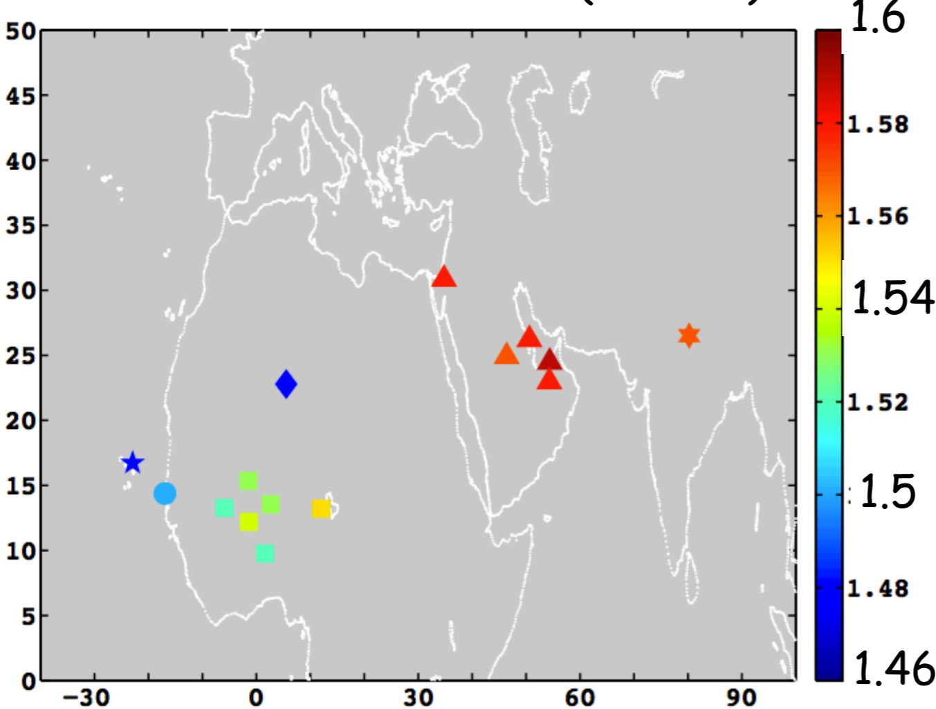
Real Refractive Index (532 nm)
