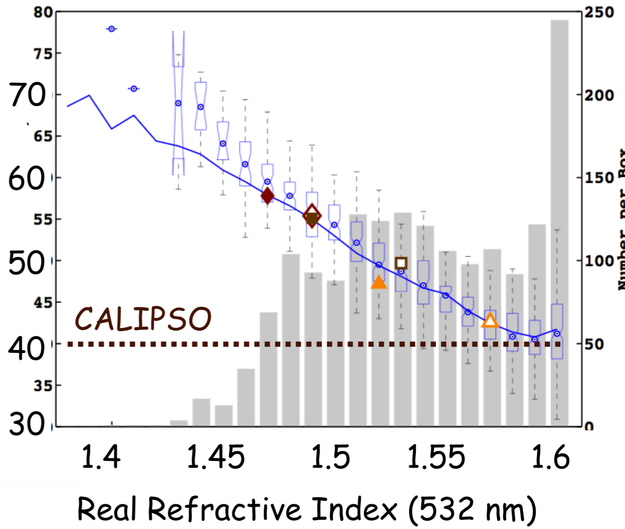
Lidar Ratio (532 nm)
