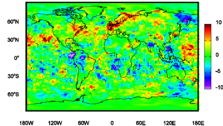
Anthropogenic aerosol effect AP - Ref (W/m 2 )
