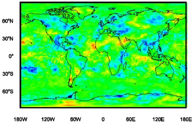
Cloud cover AP - Ref (%)
